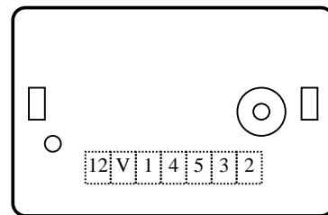
Auxiliary reader (terminal connections)
